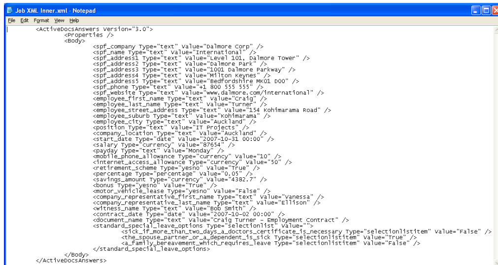
FIGURE 7 SAMPLE ANSWER DATA FOR AN EMPLOYMENT CONTRACT
